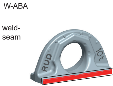
Pic. 2: area of the weld-seam changeover
