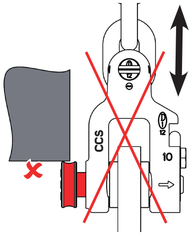
Pic. 15: Shackle pin not fully mounted
