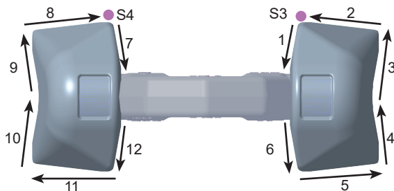
Pic. 2: Sequence of closure welding (S=Starting point)
